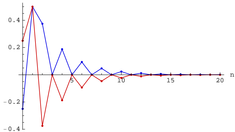
Impulse Response for K=-1/2
