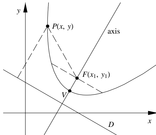
Figure 9.1: Definition of a parabola.
