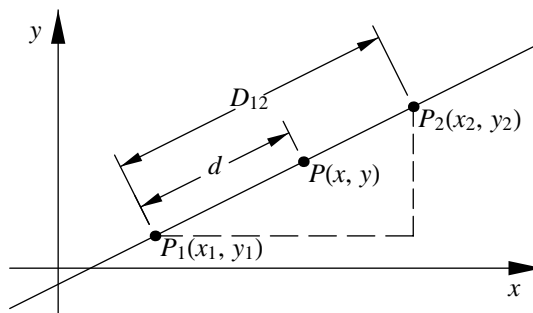
Figure 3.6: Point offset a distance towards a point.
