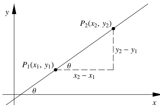
Figure 5.1: Inclination and slope of a line.
